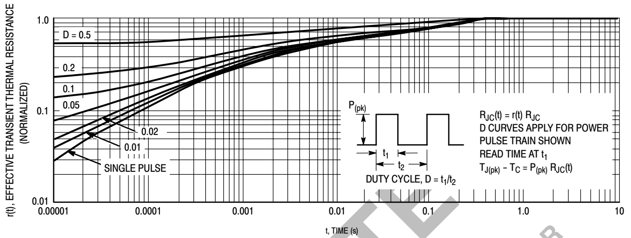
Figure 14. Thermal Response
